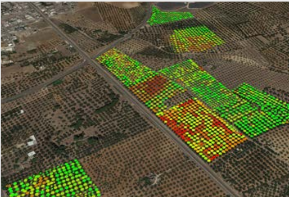
Olive trees in the Lecce Province, Apulia, Italy. Each circle represents an absolute NDVI value. The healthiest trees are colored green. The source image is from WorldView-2, processed using ENVI software.
